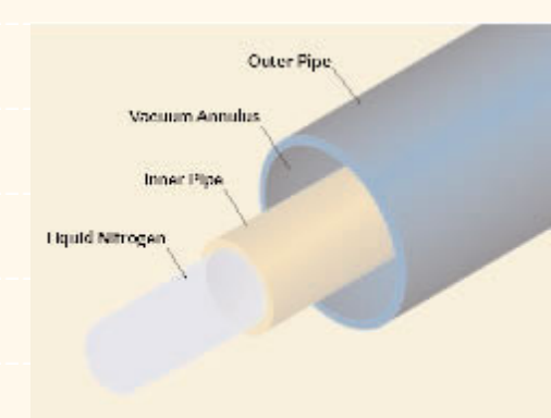
An evacuated annulus reduces conduction and convection heat losses and creates a well-insulated inner pipe for liquid nitrogen.
